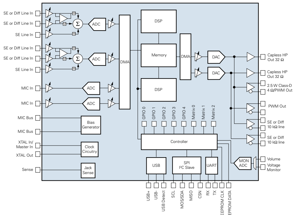
CX20706 Interface Diagram
